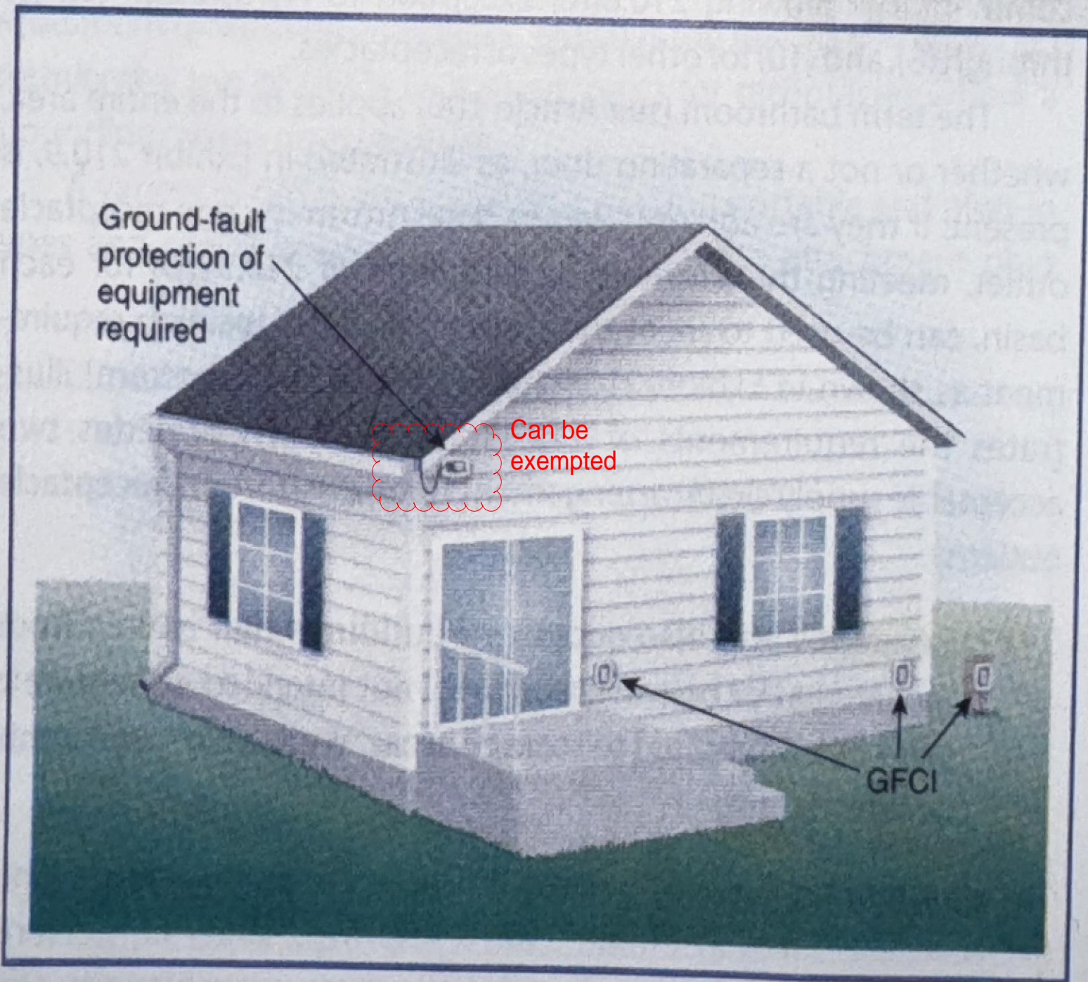
EXHIBIT 210.11 A dwelling unit with three outdoor receptacles that are required to have GFCI protection. It also has one outdoor receptacle that supplies rooftop snow melting equipment, which is protected by ground-fault protection of equipment (GFPE).
