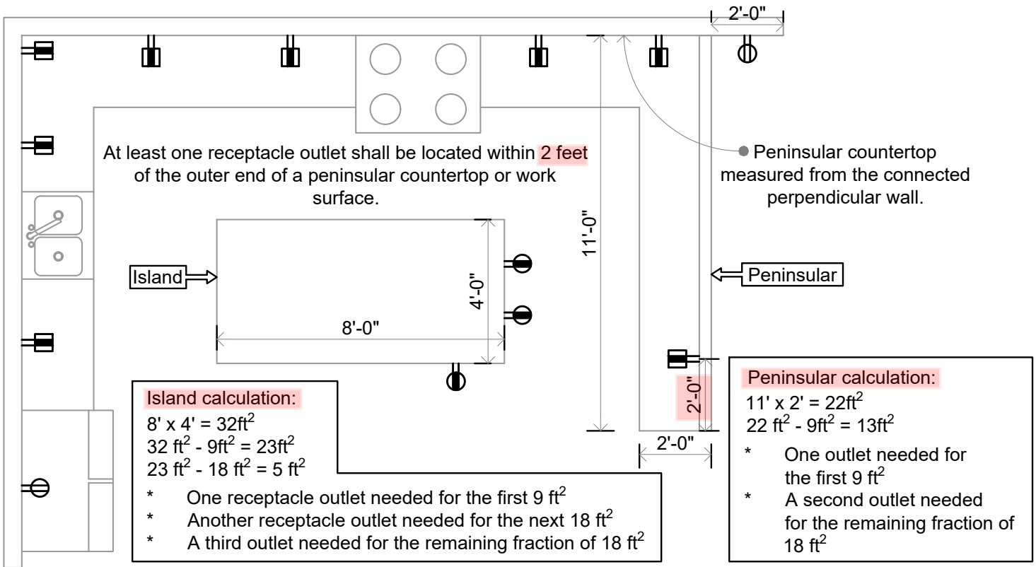
ISLAND AND PENINSULAR COUNTERTOPS AND WORK SURFACES IN ACCORDANCE WITH 210.52(C)(2)
