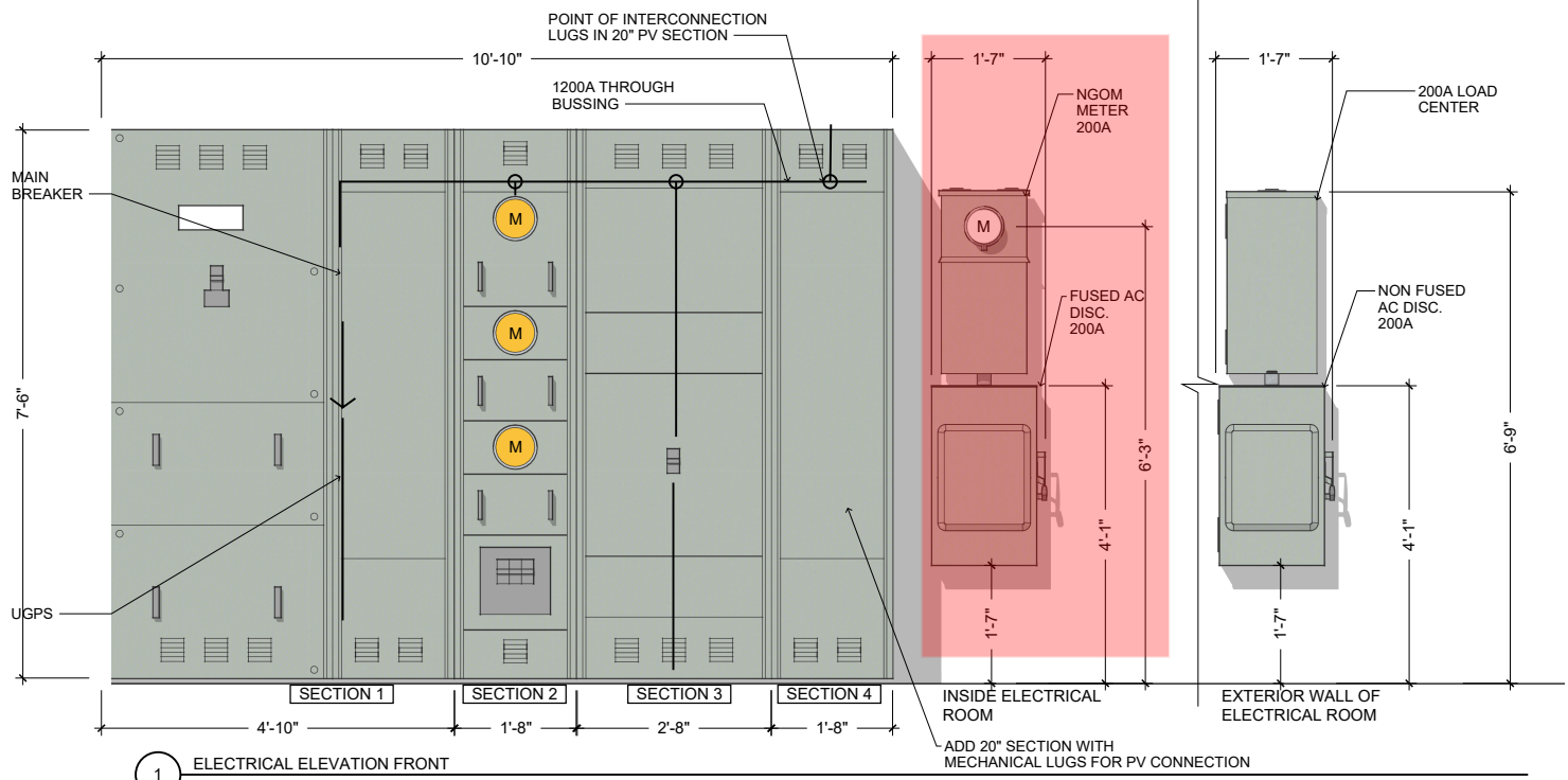
1 ELECTRICAL ELEVATION FRONT SCALE: 3/4" = 1'-0"
